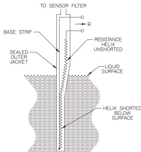
Figure 1 Sensor Operation
